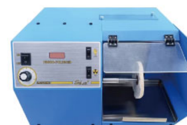
吸尘抛光机H3600 Polishing machine H3600 型号 Model: M.MT.H3600 电压 Voltage: 220V 功率 Power: 550W 尺寸 Size: 540x350x310mm 重量 Weight: 23.6KG
